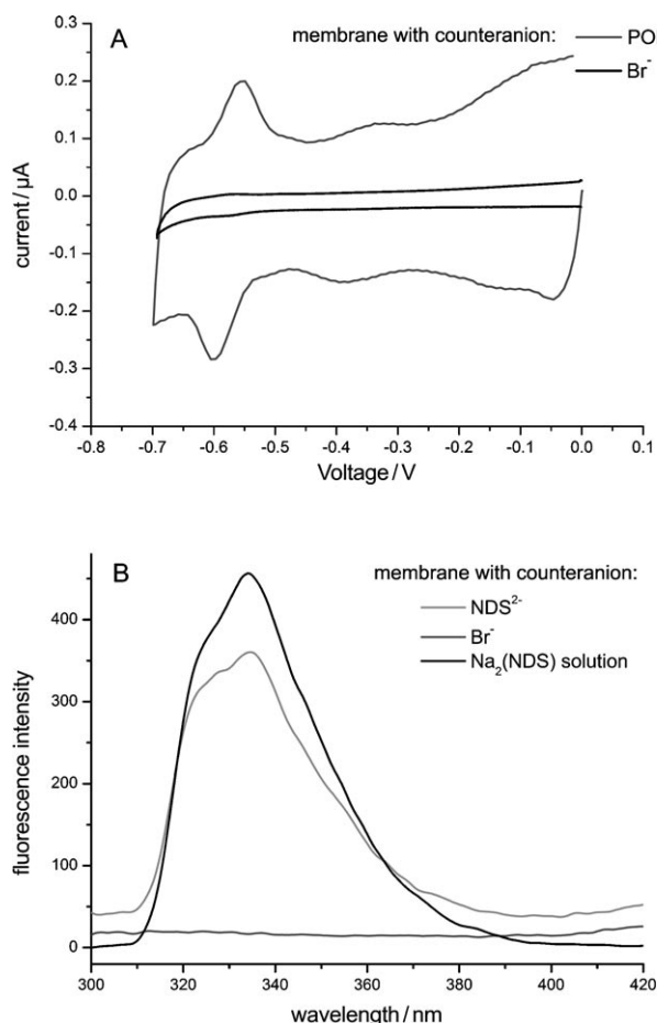
Figure 4. A) Cyclic voltammograms of the as-synthesized capsules before and after exchange with the \text{POM}^{3-} anion. B) Fluorescence spectra of the as-synthesized capsules before and after exchange with the fluorophore anion ( \text{NDS}^{2-} ) as well as of the fluorophore molecule in water.
